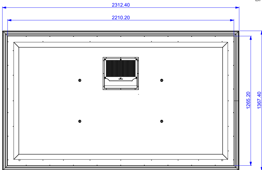
BACK
